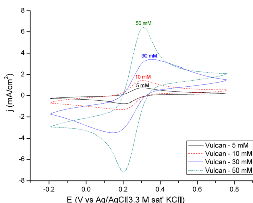
Fig. 4. Cyclic voltammograms of the Vulcan electrode with various concentrations (5, 10, 30 and 50 mM) of \text{Fe}(\text{CN})_6^{4-}/\text{Fe}(\text{CN})_6^{3-} in 1 M \text{Na}_2\text{SO}_4 .
