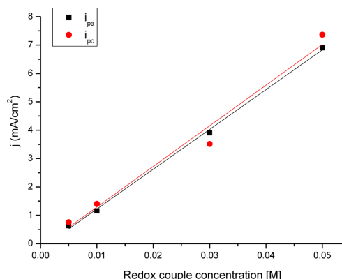
Fig. 5. Peak current densities from the cyclic voltammograms of the Vulcan electrode with various concentrations (5, 10, 30 and 50 mM) of \text{Fe}(\text{CN})_6^{4-}/\text{Fe}(\text{CN})_6^{3-} in 1 M \text{Na}_2\text{SO}_4 .
