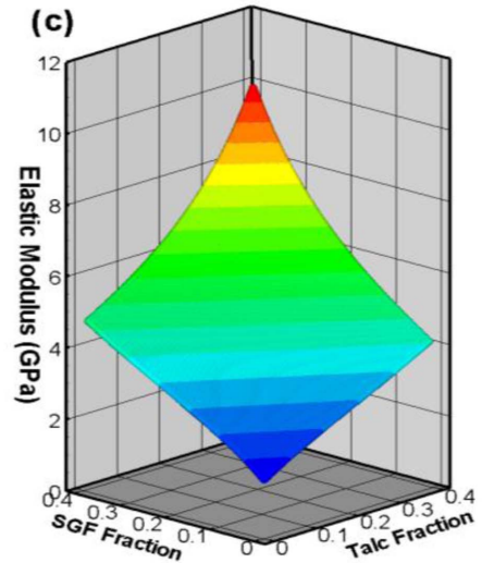
Fig. 5. Elastic moduli of hybrid composites reinforced by talc and glass fiber simultaneously. (a) Elastic moduli at constant weight fractions of talc (b) Elastic moduli at constant weight fractions of glass fiber (c) Elastic moduli predicted by the present model, i.e. Eq. (16).
