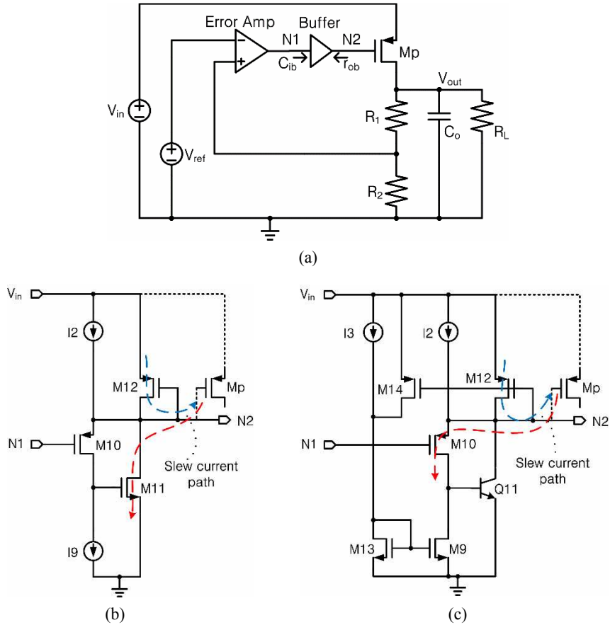
Fig. 1. Schematic of LDO (a) with a buffer, (b) proposed buffer circuit, (c) reported buffer circuit [1].
