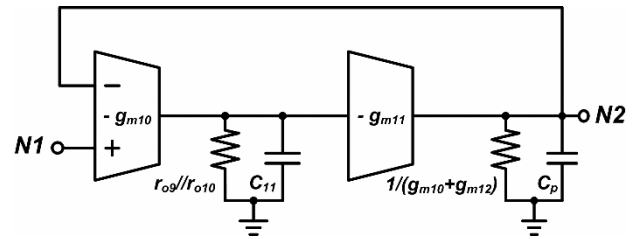
Fig. 3. Small signal model of the proposed buffer.
