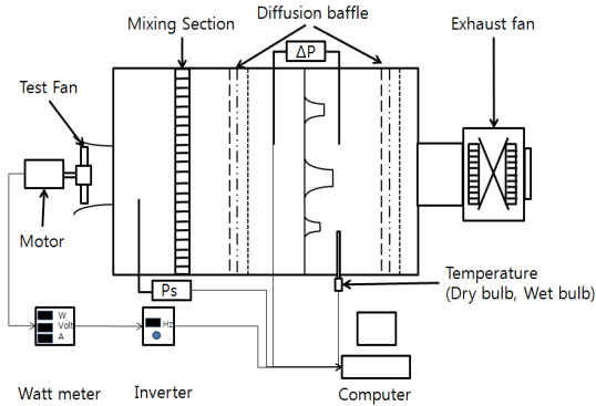
[Fig. 2] Air Flow Measurement System
