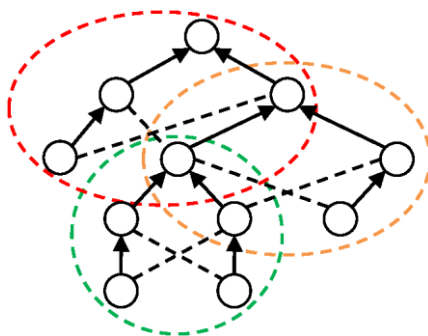
Fig. 8. The overlapped \mathbb{C}\mathbb{S}_n . Each ellipse contains a \mathbb{C}\mathbb{S}_n .
