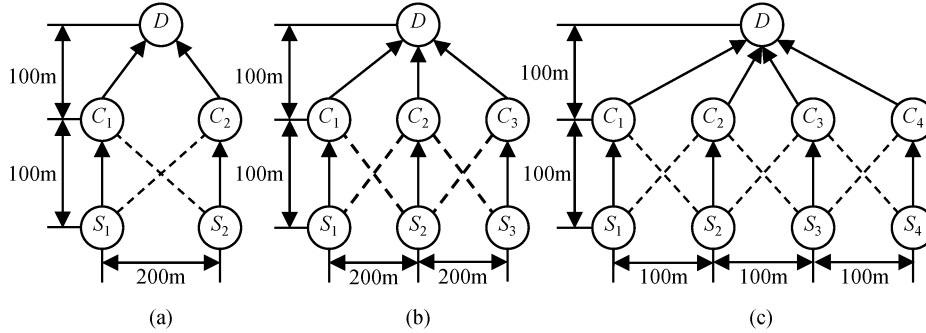
Fig. 7. network topologies for simulations, (a) for CS_2 , (b) for CS_3 , (c) for CS_4 .
