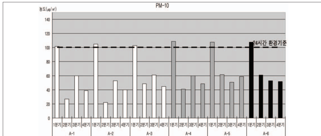
Fig. 2. Seasonal Concentrations of PM-10
