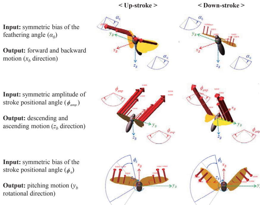
Fig. 6. Aerodynamic vectors on the wings under longitudinal control inputs
