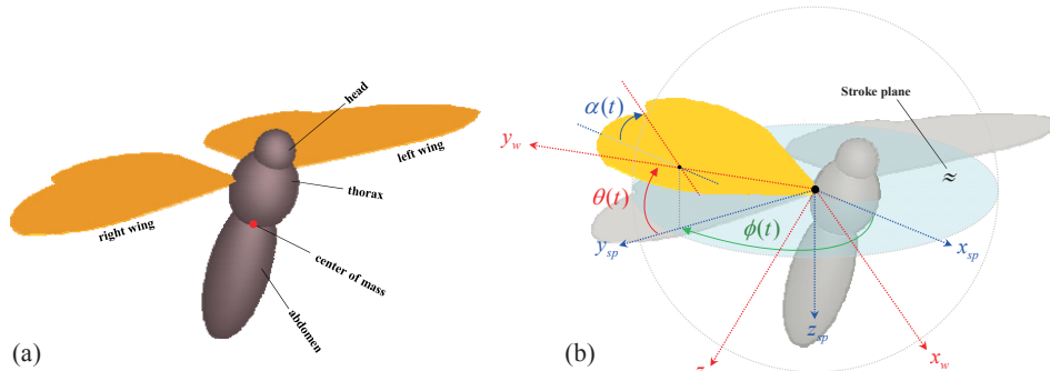
Fig. 1. (a) Multibody dynamics model of the hawkmoth, where each body component (head, thorax, and abdomen) is modeled as an ellipsoid of revolution, (b) Definition of the wing kinematics: \phi(t) , positional angle; \alpha(t) , feathering angle; and \theta(t) , deviation angle.
