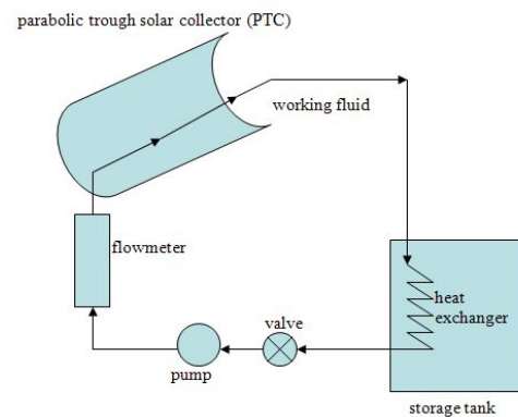
Fig. 1 Systematic of parabolic trough collector.
