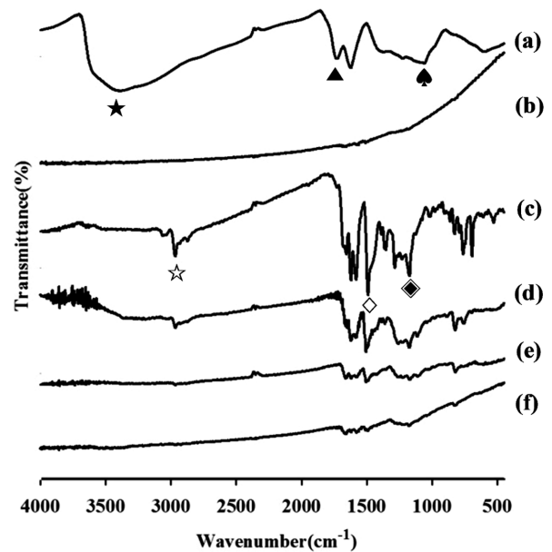
Figure 1. FTIR spectra of (a) GO; (b) TRGO; (c) PBZ; (d) G-PBZ-1; (e) G-PBZ-2; (f) G-PBZ-3.
