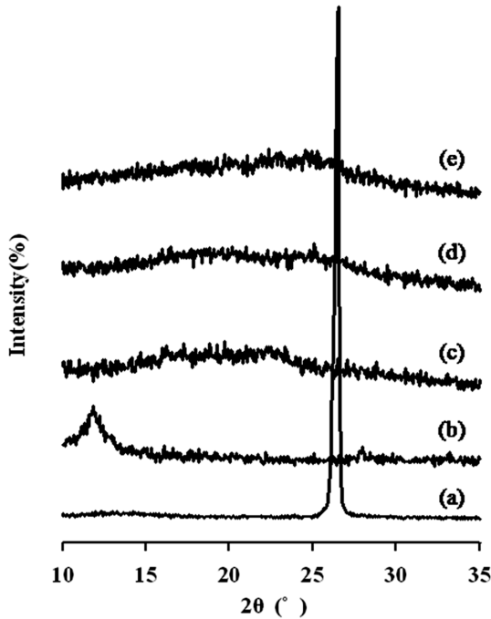
Figure 2. XRD patterns of (a) graphite; (b) GO; (c) G-PBZ-1; (d) G-PBZ-2; (e) G-PBZ-3.
