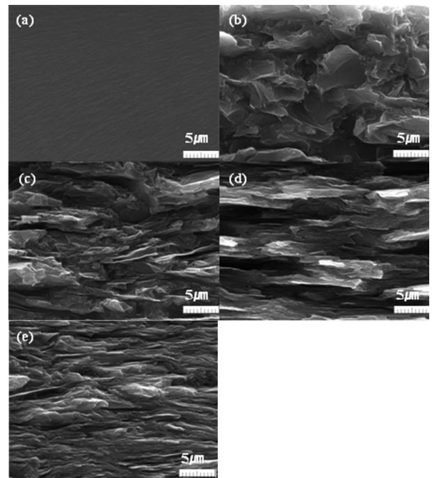
Figure 3. Cross-sectional SEM images of (a) PBZ; (b) G-PBZ-1; (c) G-PBZ-2; (d) G-PBZ-3; (e) G-PBZ-4.
