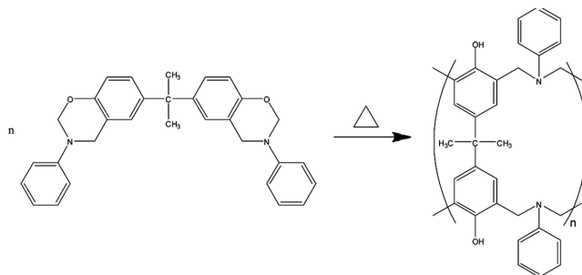
Scheme 1. Typical thermal inducing ring-opening polymerization mechanism of bisphenol-A type benzoxazine (BZ).
