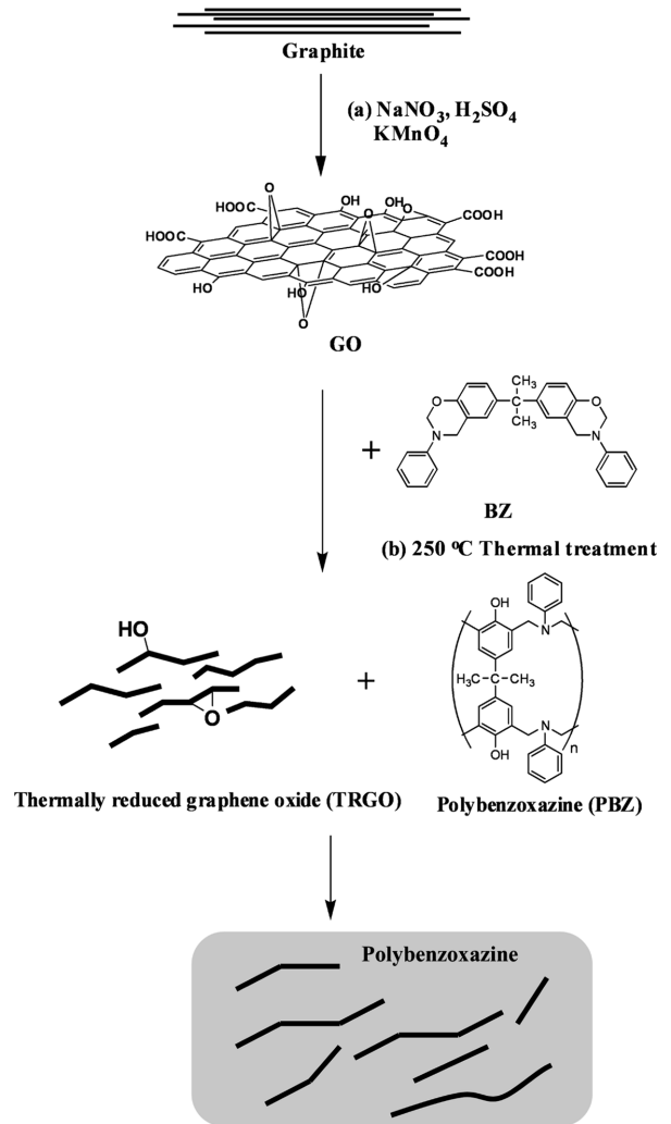
Scheme 2. Plausible preparation route of graphene/PBZ nano composite.
