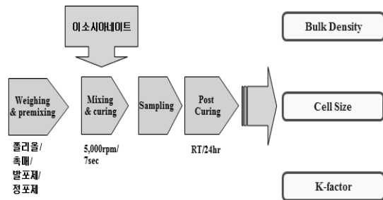
[Fig. 2] Schematic diagram of sample fabrication process for open-celled rigid PUF.
