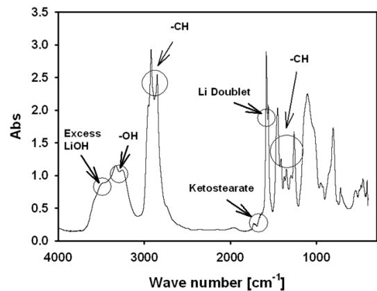
[Fig. 3] FT-IR spectrum of Li-12HSA dispersed in silicone oil.
