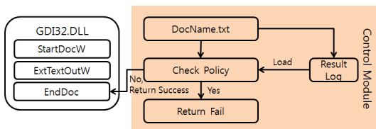
[Fig. 6] Print Control System of Personal Information
