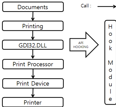
[Fig. 1] API Hooking Method
