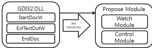
[Fig. 2] Composition of the Proposed Module
