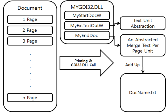
[Fig. 3] Character String Extraction System
