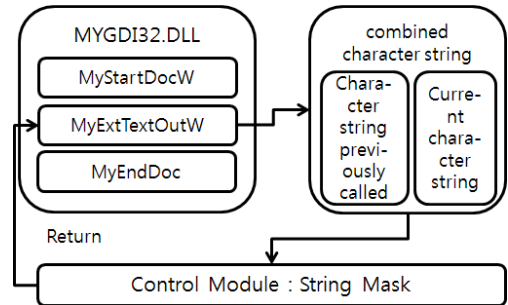
[Fig. 7] Character String Mask System of Personal Information
