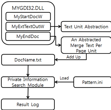
[Fig. 5] Personal Information Detection System
