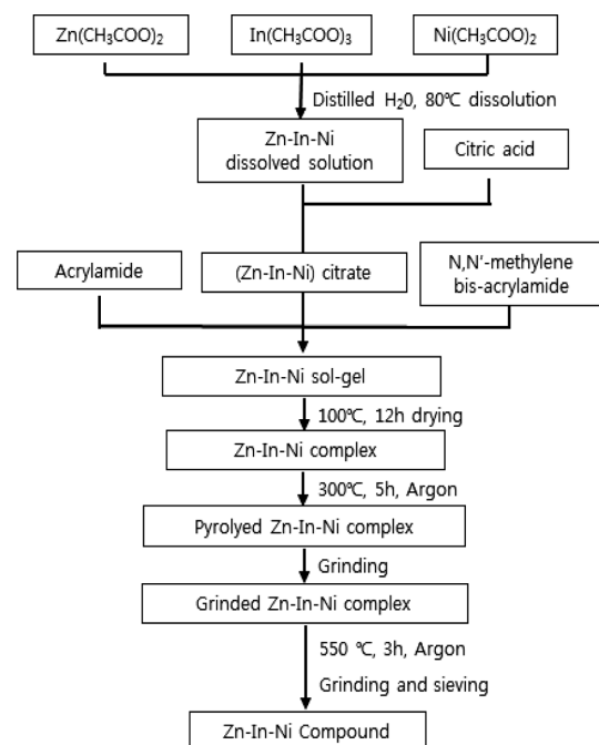
Fig. 1. Synthetic scheme of Zn-In-Ni composite compounds by citric acid modified Sol-Gel method.
