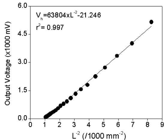
Fig. 2. Relationship between the output voltage (Vh) of the Hall element sensor and the distance (L=Lc+8.5 mm La: 5.0 mm, Lb: 3.5 mm) from the Hall element sensor on the left valve to the magnet on the right valve.
