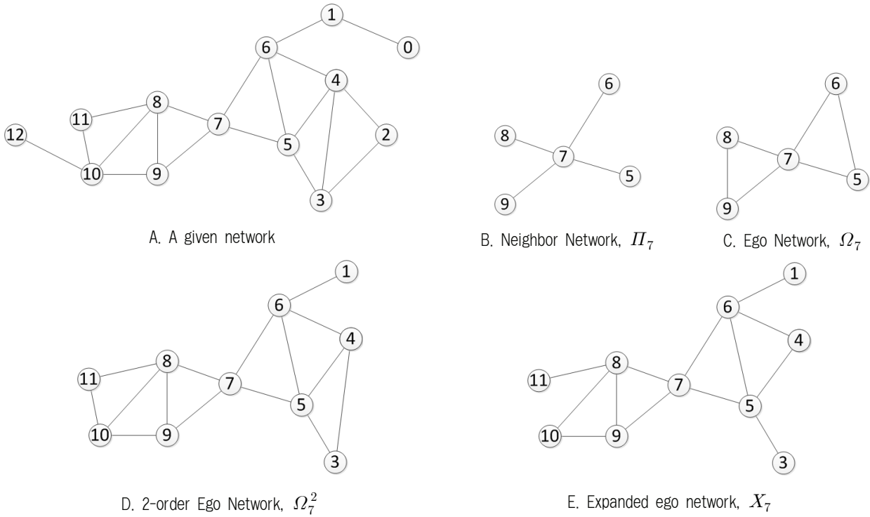
Fig. 1. A given network and the node v_7 's neighbor, ego, 2-order ego, and expanded ego networks
