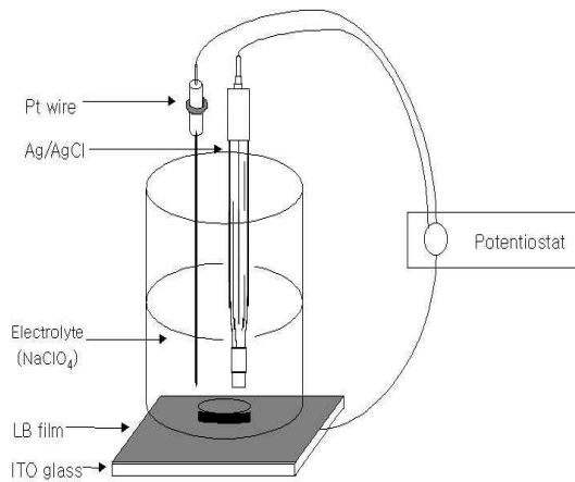
Fig. 2. The cell of electrochemical measuring equipment.
