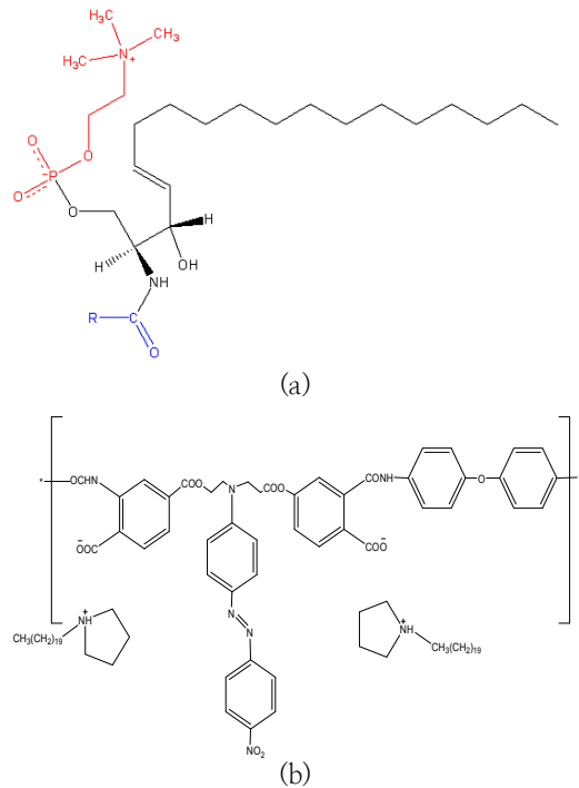
Fig. 1. Molecular structures of the (a) sphingomyelin and (b) polyamic acid salt.
