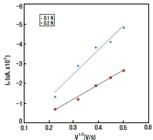
Fig. 6. Plot of i_p vs v^{1/2} of polyamic acid phospholipid mixture LB films.
