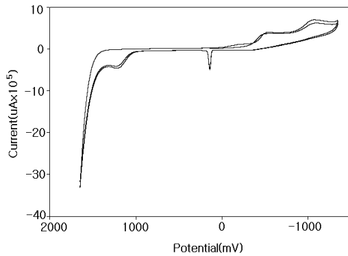
Fig. 4. Cyclic voltammogram for mono-layer sphingomyelin and polyamic acid(1:1) mixture on an ITO electrode in 0.1 N \text{KClO}_4 solution.
