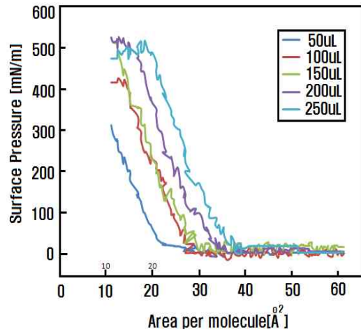
Fig. 3. \pi -A curves of sphingomyelin and polyamic acid mixture.
