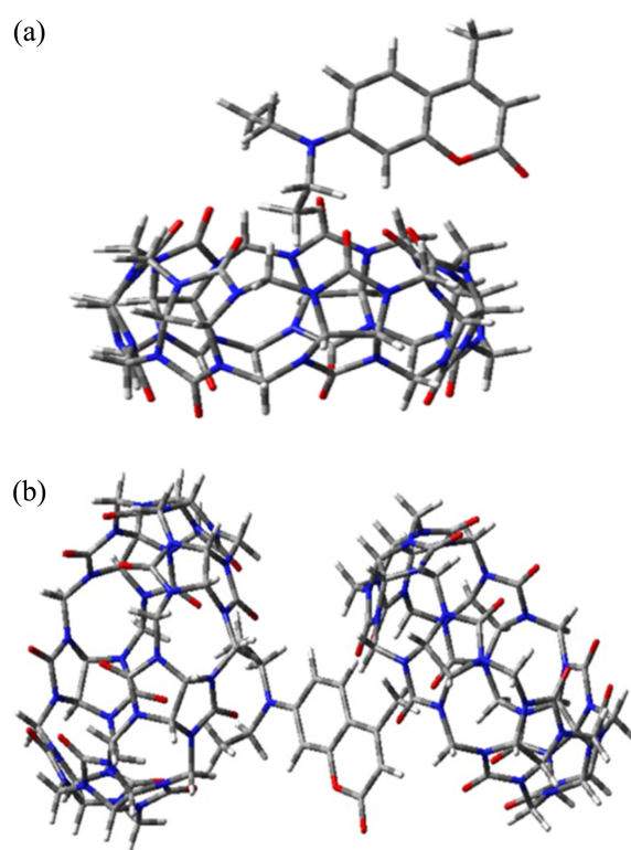
Figure 5. Optimized structures for (a) 1:1 complex and, (b) 2:1 complex calculated with AM1 semi-empirical method.
