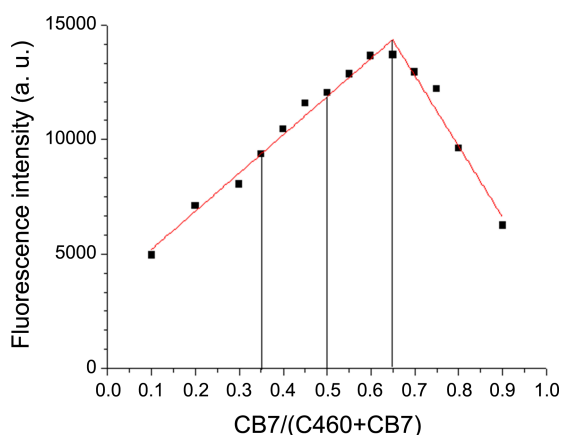
Figure 4. Job's plots obtained for C460-CB7 complexes. The maximum fluorescence intensity is obtained at about 0.65 mole fraction of CB7.
