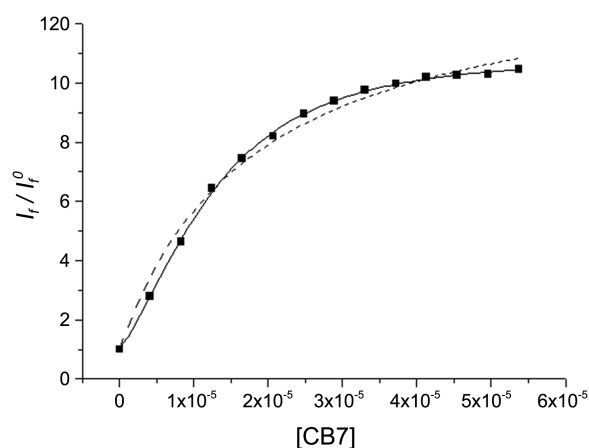
Figure 3. Fluorescence enhancement of C460 as a function of CB7 concentration. The solid line represents the best fit for the 2:1 stoichiometry using Eq. (2) and the dashed line represents 1:1 stoichiometry using Eq. (1).
