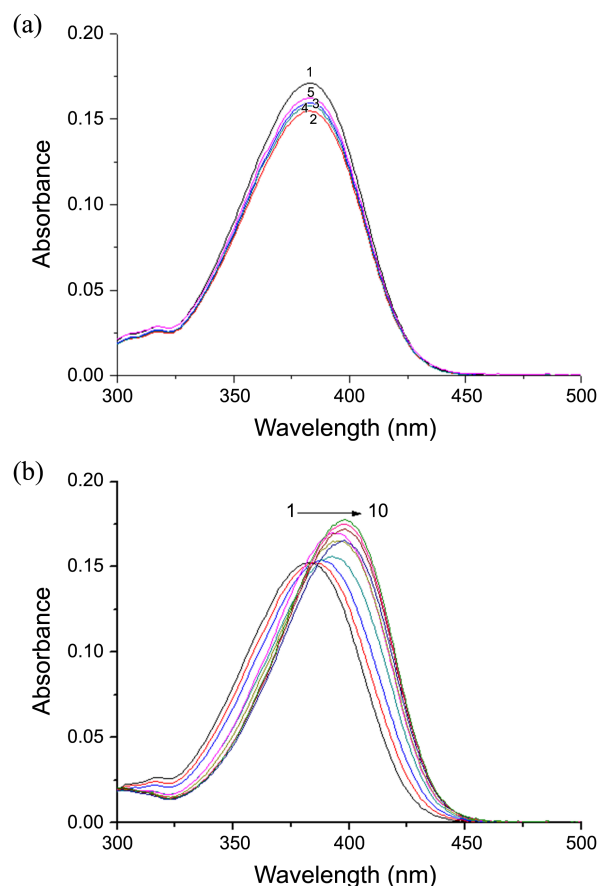
Figure 1. (a) UV/Vis absorption spectra of C460 with various concentrations of CB6. (1) no CB6, (2) 6.25 mM, (3) 1.25 mM, (4) 4.38 mM, (5) 7.50 mM, (b) UV/Vis absorption spectra of C460 with various concentrations of CB7. (1) no CB7, (2) 4.13 mM, (3) 8.26 mM, (4) 12.4 mM, (5) 20.7 mM, (6) 24.8 mM, (7) 41.3 mM, (8) 45.4 mM, (9) 49.6 mM, (10) 54.7 mM.
