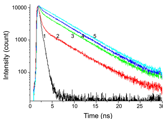
Figure 6. Fluorescence lifetime measurements for C460 with the addition of CB7. The average fluorescence lifetime increases with CB7 concentration. (1) no CB7, (2) 4.13 mM, (3) 8.26 mM, (4) 12.4 mM, (5) 54.7 mM.
