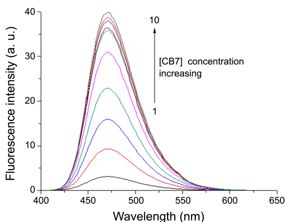
Figure 2. Fluorescence intensity change of C460 with the incremental addition of CB7. (1) no CB7, (2) 4.13 mM, (3) 8.26 mM, (4) 12.4 mM, (5) 20.7 mM, (6) 24.8 mM, (7) 41.3 mM, (8) 45.4 mM, (9) 49.6 mM, (10) 54.7 mM.
