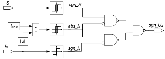
Fig. 3. Diagram block of the current limiter integration in the switching law.
