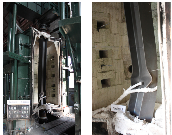
Fig. 4 The failure mode of test model C(S-3)
