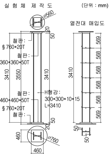
(c) Manufacture drawing of test model
