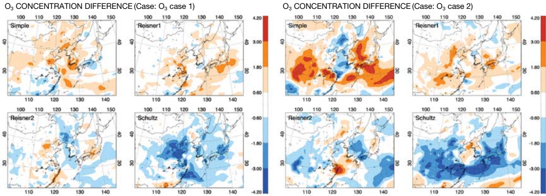
Fig. 11. Horizontal distributions of difference of O 3 concentration arising from selecting different microphysics for the chosen two cases.
