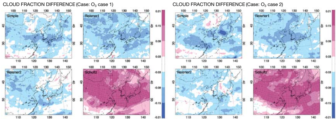
Fig. 12. Horizontal distributions of difference of cloud fraction arising from selecting different microphysics for the chosen two cases.
