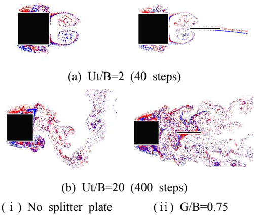
Figure 9: Vortex distributions around square prism without and having splitter plate
