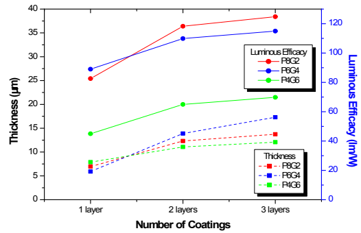
Fig. 3. Thickness and luminous efficacy according to number of coatings.
