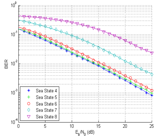
Fig. 5. simulation results for the effect of ship rocking on the BER performance with different sea state conditions for small sized ship
