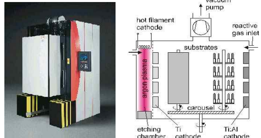
Fig.1. Balzers BAT1200 coating system and PVD coating mechanism.
