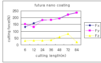
(a) futura nano coating
