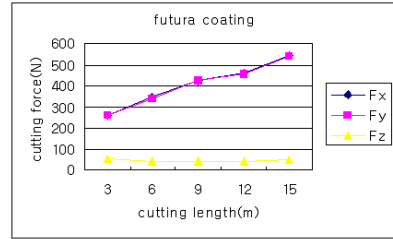
(b) futura coating
