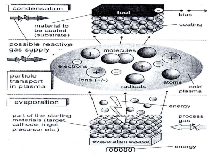
Fig.2. The three phases of coating formation.
