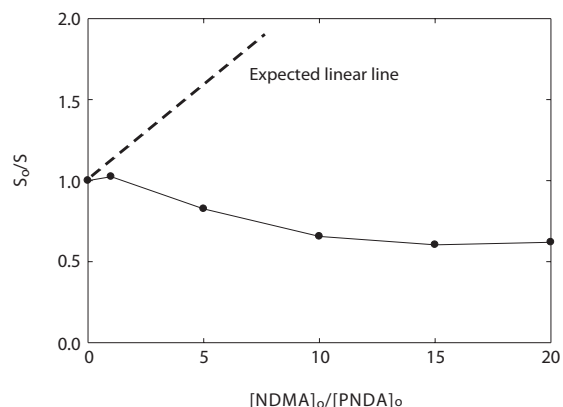
Fig. 4. S_0/S plotted against [\text{NDMA}]_0/[\text{PNDA}]_0 . Experimental conditions: pH, 8.75; [\text{H}_2\text{O}_2]_0 = 10 \mu\text{M} , [\text{PNDA}]_0 = 2 \mu\text{M} ; and wavelength, 254 nm. Note that the dashed line is a linear line generally expected in the competition kinetics. NDMA: N-nitrosodimethylamine, PNDA: p-nitrosodimethylaniline.
