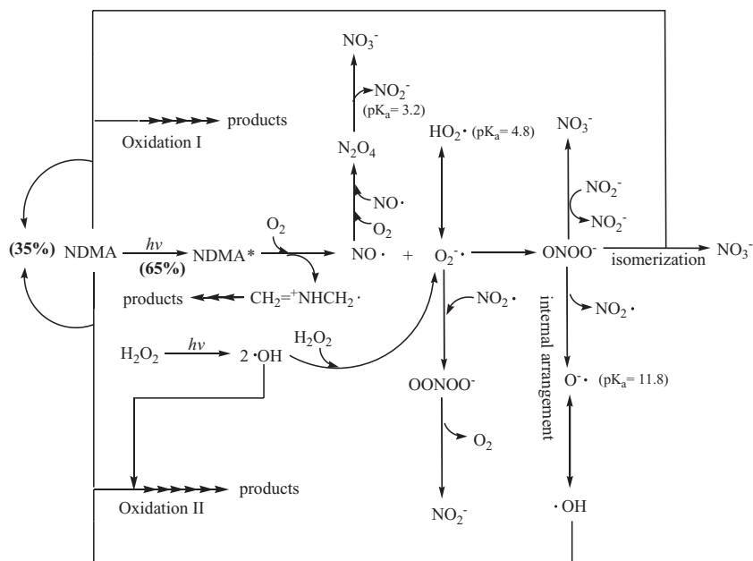
Fig. 3. Mechanism of the photolytic pathways for formation of URS during NDMA photolysis in the presence of \text{H}_2\text{O}_2 . Note that the percentage in parentheses shows the contribution of the reactive species (or URS) and UV photolysis, respectively, on NDMA degradation. NDMA: N-nitrosodimethylamine, URS: unknown reactive species.
