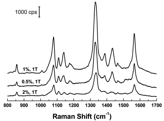
Fig. 4. Surface enhanced Raman spectrum from a single silica@Au microspheres modified with NBT as a function of the concentration of APTES (w/v). '1T' denotes single step of electroless plating.
