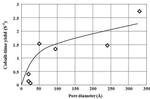
Fig. 12. Cobalt-time yield as a function of pore sizes [23].
