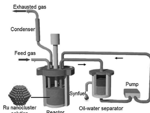
Fig. 9. Scheme of continuous flow reactor for the aqueous phase FTS [16].
