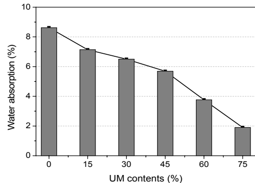
[Fig. 4] Test results of water absorption ratio
