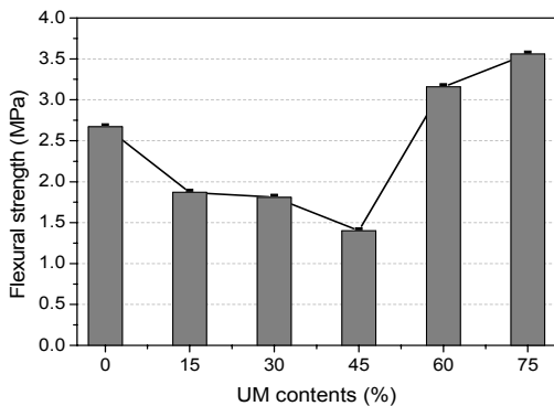
[Fig. 3] Test results of flexural strength
