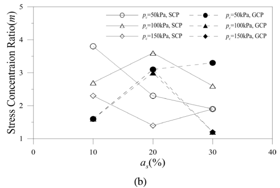
[Fig. 7] m - a_s relationships
