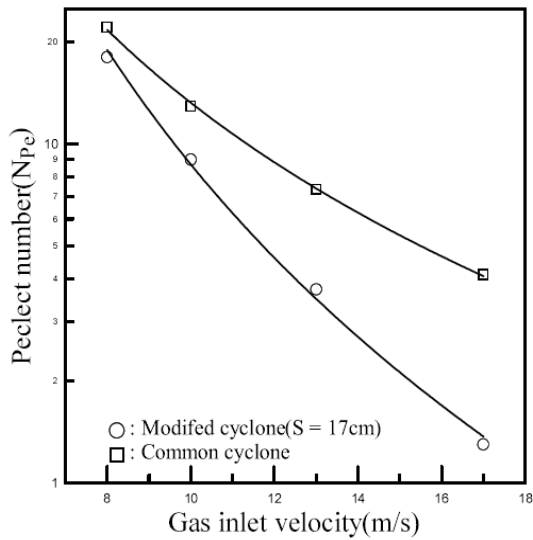
[그림 9] N_{Pe} of glass bead flow in a common and modified cyclone(S = 17cm) with inlet gas velocity.
