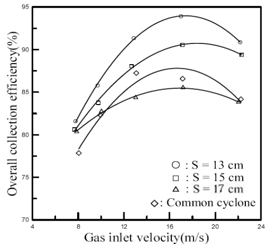
[Fig. 4] Overall collection efficiency of fly ash in a modified and common cyclone with gas inlet velocity.
