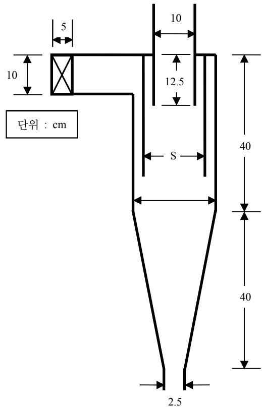
[Fig. 1] Geometric ratio of modified cyclone.
