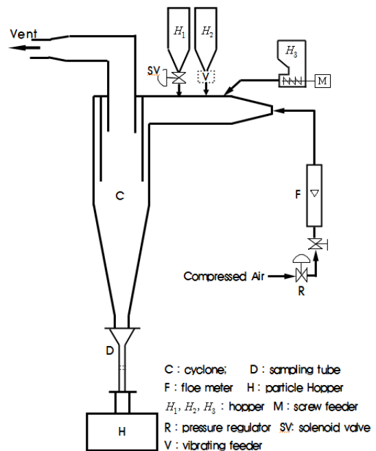
[Fig. 2] Schematic diagram of experimental apparatus.
