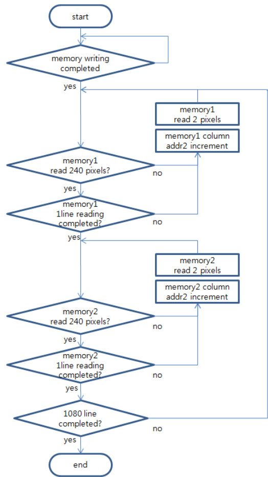
[Fig. 6] Flowchart of memory reading operation at side by side mode
