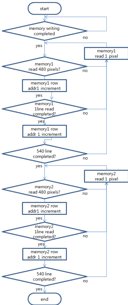
[Fig. 5] Flowchart of memory reading operation at top and bottom mode
