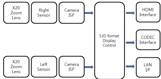
[Fig. 2] Block Diagram of Stereo Camera
