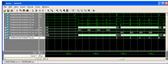
[Fig. 10] Simulation result1 of memory writing operation- row address and bank address
