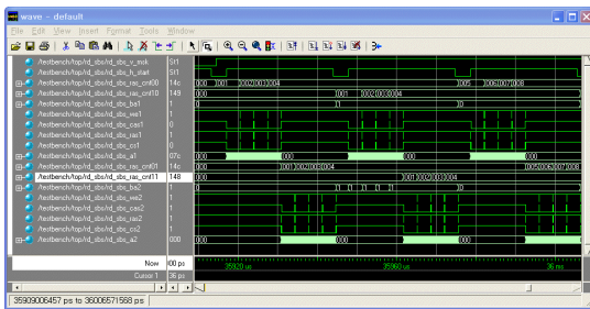
[Fig. 11] Simulation result of memory reading operation at side by side mode - row address
