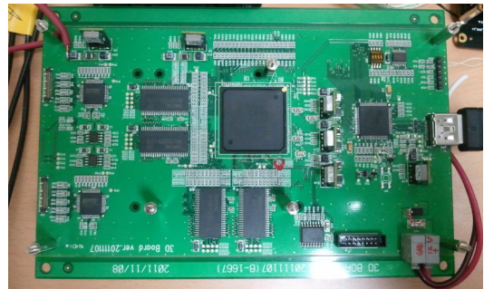
[Fig. 8] Stereo Camera Board
