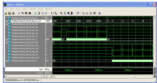
[Fig. 13] Simulation result of memory reading operation at top and bottom mode - row address and bank address
