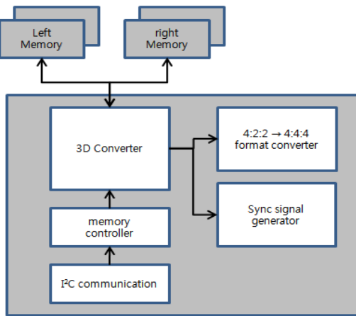
[Fig. 3] Block Diagram of Stereo Format Converter
