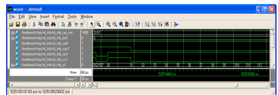
[Fig. 14] Simulation result of memory reading operation at top and bottom mode - column address
