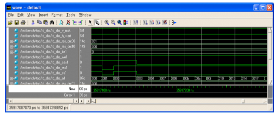
[Fig. 12] Simulation result of memory reading operation at side by side mode - column address
