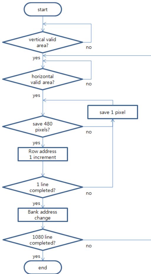
[Fig. 4] Flowchart of memory writing operation
