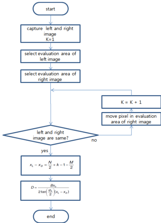
[Fig. 7] Flowchart of measuring depth of object
