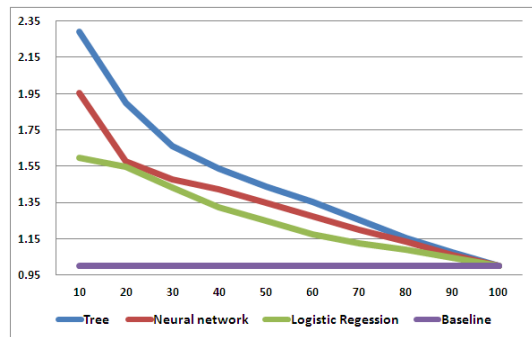
[Fig. 1] Model assessment using lift graph
