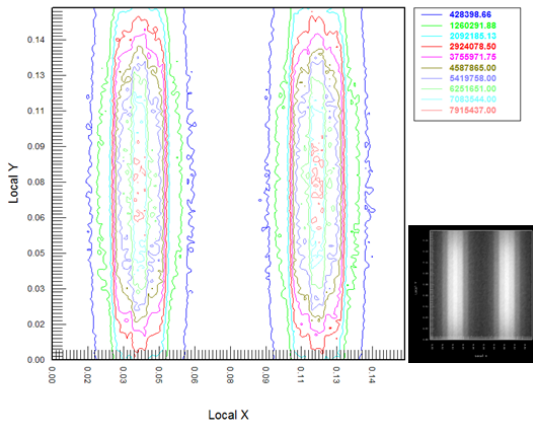
[Fig. 7] Illuminance distribution for optimal reflector
