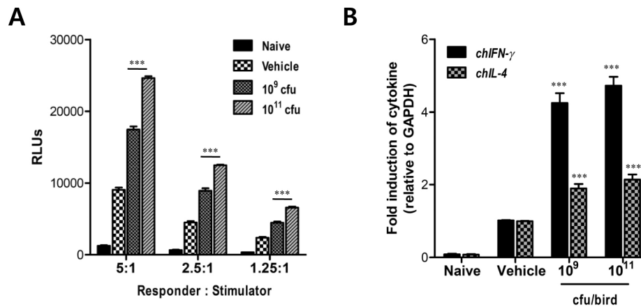
Figure 4. Enhanced Th1-biased immunity in chickens vaccinated with inactivated NDV (B1 strain) vaccine following oral administration of S. enterica serovar Typhimurium expressing chIL-18. (A) NDV (B1 strain) antigen-specific proliferation of PBMCs. Groups of chickens were administered S. enterica serovar Typhimurium expressing chIL-18 ( 10^9 and 10^{11} cfu/chicken) and vaccinated with inactivated NDV (B1 strain) vaccine three days later. The vaccination was performed by same protocol twice at 7-day intervals. PBMCs (responders) were prepared from chickens 14 days after booster vaccination, and subsequently stimulated with autologous naïve PBMCs (stimulators) that had been pulsed with uv-inactivated NDV (B1 strain) antigen. Antigen-specific proliferation of PBMCs was assessed by measuring viable cell ATP bioluminescence following incubation for 72 h. (B) The expression of IFN- \gamma and IL-4 mRNA by PBMCs following stimulation with NDV (B1 strain) specific antigen. Total RNA was extracted from PBMCs stimulated with specific antigen for 72 h, and subjected to real-time qRT-PCR to determine the expression of IFN- \gamma and IL-4. Data show the average and SEM of IFN- \gamma and IL-4 expression obtained from six chickens per group, after normalized to GAPDH. *** p < 0.001 compared to vehicle group treated with control bacteria.
