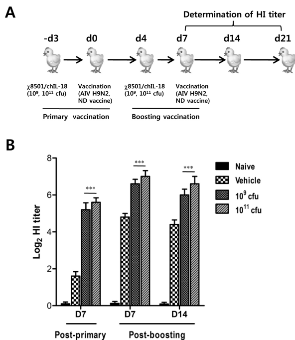
Figure 1. The serum hemagglutination inhibition (HI) antibody titers in chickens vaccinated intramuscularly with inactivated AIV H9N2 vaccine with or without oral administration of S. enterica serovar Typhimurium expressing chIL-18. (A) Diagram for vaccination schedule using S. enterica serovar Typhimurium expressing chIL-18. Groups of chickens administered S. enterica serovar Typhimurium expressing chIL-18 ( 10^9 and 10^{11} cfu/chicken) and vaccinated with inactivated AIV H9N2 vaccine three days later. The vaccinations were performed by same protocol twice at 7-day intervals. (B) HI antibody titers in sera of vaccinated chickens. Serum samples collected from chickens of all groups 7 days after primary vaccination and 7 and 14 days after booster vaccination were subjected to HI testing. Data are expressed as reciprocal log 2 of the geometric average and SEM of HI titers obtained from five chickens per group. ***p < 0.001 compared to vehicle group treated with control bacteria.
