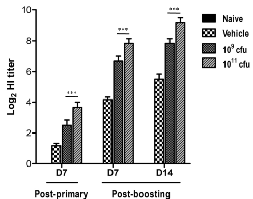
Figure 2. The serum hemagglutination inhibition (HI) antibody titers in chickens vaccinated intramuscularly with inactivated NDV (B1 strain) vaccine with or without oral administration of S. enterica serovar Typhimurium expressing chIL18. Groups of chickens were administered S. enterica serovar Typhimurium expressing chIL-18 ( 10^9 and 10^{11} cfu/chicken) and vaccinated with inactivated NDV (B1 strain) vaccine three days later. The vaccinations were performed by same protocol twice at 7-day intervals. Serum samples collected from chickens of all groups 7 days after primary vaccination and 7 and 14 days after booster vaccination were subjected to HI testing. Data are expressed as reciprocal log 2 of the geometric average and SEM of HI titers obtained from six chickens per group. ***p < 0.001 compared to vehicle group treated with control bacteria.
