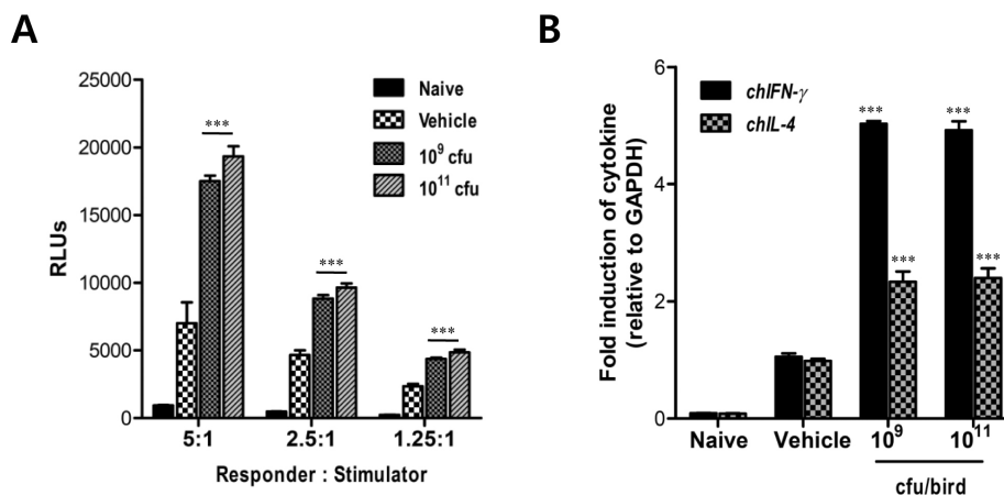
Figure 3. Enhanced Th1-biased immunity in chickens vaccinated with inactivated AIV H9N2 vaccine following oral administration of S. enterica serovar Typhimurium expressing chIL-18. (A) AIV H9N2 antigen-specific proliferation of PBMCs. Groups of chickens were administered S. enterica serovar Typhimurium expressing chIL-18 ( 10^9 and 10^{11} cfu/chicken) and vaccinated with inactivated AIV H9N2 vaccine three days later. The vaccination was performed by same protocol twice at 7-day intervals. PBMCs (responders) were prepared from chickens 14 days after booster vaccination, and subsequently stimulated with autologous naive PBMCs (stimulators) that had been pulsed with uv-inactivated AIV H9N2 antigen. Antigen-specific proliferation of PBMCs was assessed by measuring viable cell ATP bioluminescence following incubation for 72 h. (B) The expression of IFN- \gamma and IL-4 mRNA by PBMCs following stimulation with AIV H9N2 specific antigen. Total RNA was extracted from PBMCs stimulated with specific antigen for 72 h, and subjected to real-time qRT-PCR to determine the expression of IFN- \gamma and IL-4. Data show the average and SEM of IFN- \gamma and IL-4 expression obtained from five chickens per group, after normalized to GAPDH. *** p < 0.001 compared to vehicle group treated with control bacteria.
