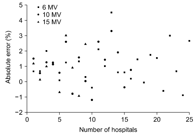
Fig. 4. Distribution of outputs for 6, 10, and 15 MV photon beams performed in 25 hospitals.
