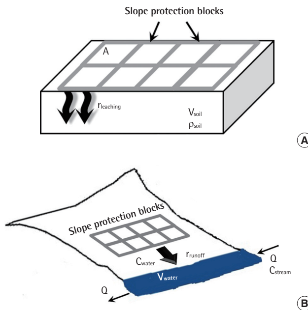
Figure 1. Schematic diagram of the exposure model for the risk assessment of chemicals released from slope protection blocks in the (A) soil compartment and (B) stream segment.
