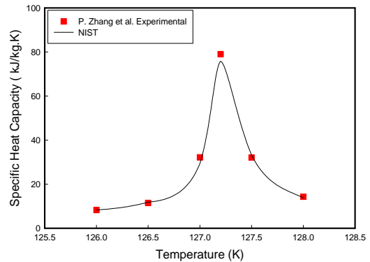
Figure 2: Comparison of NIST database material of nitrogen with P. Zhang et al. [5] data's.
