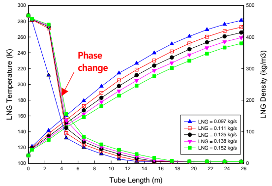
(b) LNG Temperature distributions in case of Glycol Water mass flow rate 1.805 kg/s Figure 6: Temperature distribution of LNG
