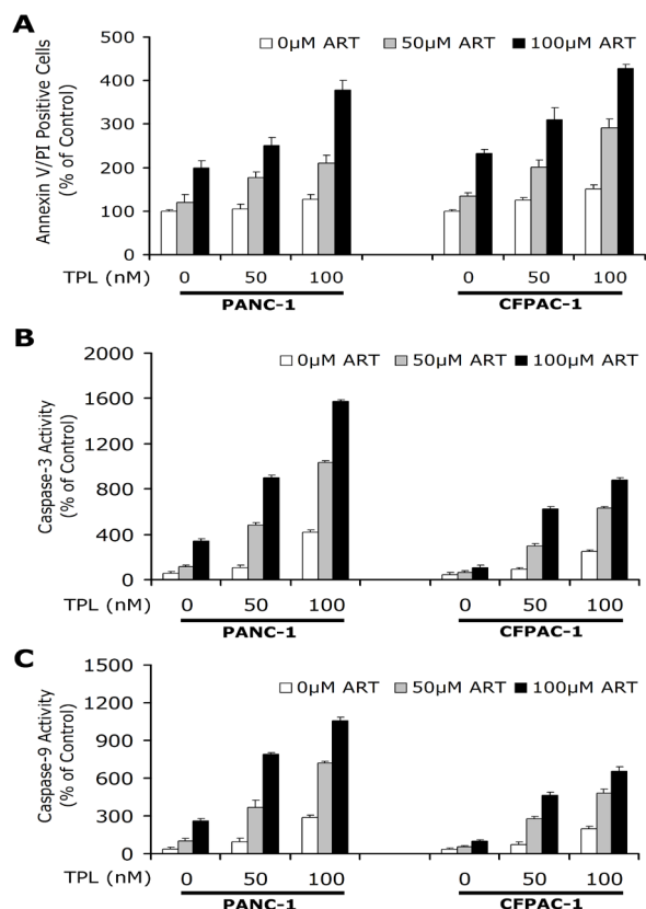
Figure 2. Triptolide and Artesunate Combination Induce PANC-1 and CFPAC-1 Cells Apoptosis and Caspase Activation. The presence of 50 and 100 nM of triptolide and 50 and 100 μM of artesunate in the culture medium for 24 h significantly induced both PANC-1 and CFPAC-1 cells apoptosis (A). Activity of caspase-3 (B) and caspase-9 (C) in PANC-1 and CFPAC-1 cells treated with triptolide and artesunate alone or in combination for 24 h
