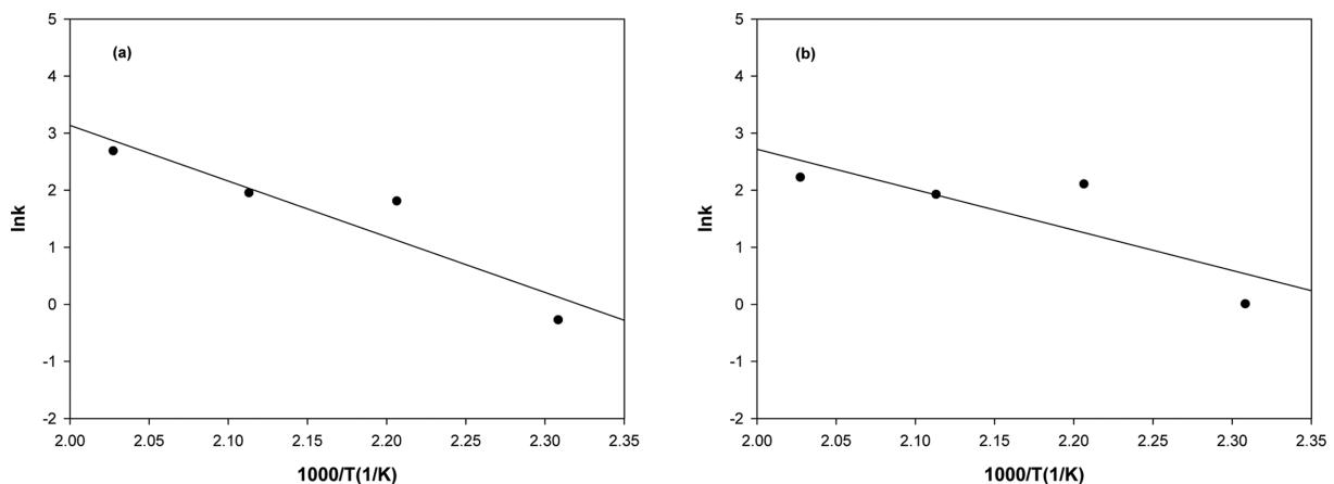
Fig. 7. Arrhenius plot for transesterification of methyl ester group to hydroxyl ethyl ester group: (a) reaction from methylester end group to hydroxylethyl ester end group; (b) reaction from hydroxylethyl ester end group to methyl ester end group.
