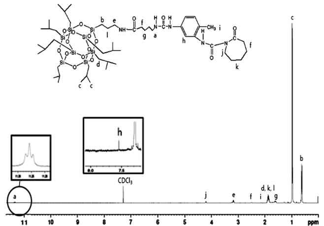
Figure 3. 1 H NMR spectrum of POSS-(TDI+CL).
