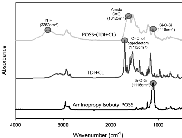
Figure 2. FTIR spectra of aminopropyl isobutyl POSS, TDI+CL, and POSS-(TDI+CL).
