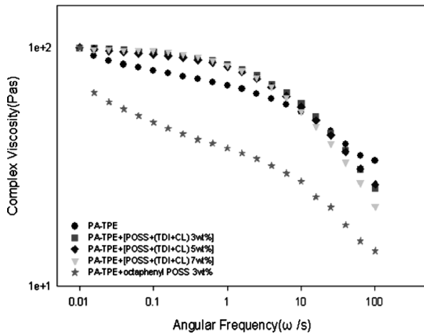
Figure 8. Complex viscosity vs. angular frequency of PEBA4033/POSS-(TDI+CL) composites with different POSS-(TDI+CL) contents and PA-TPE/octaphenyl POSS.
