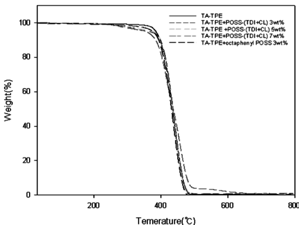
Figure 5. TGA thermograms of PA-TPE/POSS-(TDI+CL) composites with different POSS-(TDI+CL) contents and PA-TPE/octaphenyl POSS.
