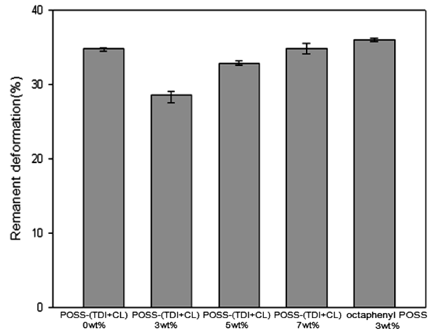
Figure 7. Tension set of PA-TPE/POSS-(TDI+CL) composites with different POSS-(TDI+CL) contents and PA-TPE/octaphenyl POSS.
