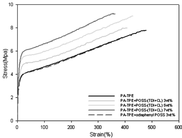
Figure 6. Stress-strain curves of PA-TPE/POSS-(TDI+CL) composites with different POSS-(TDI+CL) contents and PA-TPE/octaphenyl POSS.
