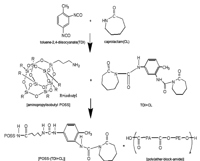
Figure 1. Reaction process of POSS-(TDI+CL) and PA-TPE/POSS-(TDI+CL) composite.
