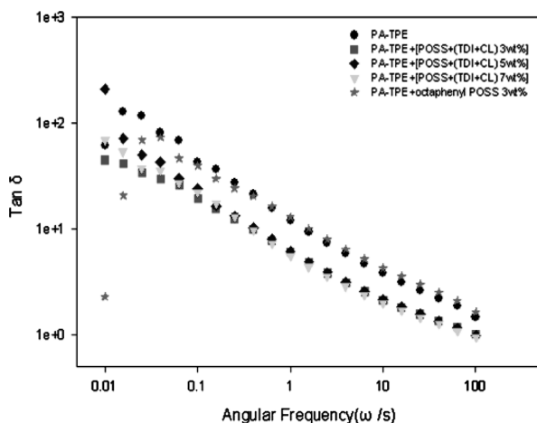
Figure 9. Tan \delta vs. angular frequency of PA-TPE/POSS-(TDI+CL) composites with different POSS-(TDI+CL) contents and PA-TPE/octaphenyl POSS.
