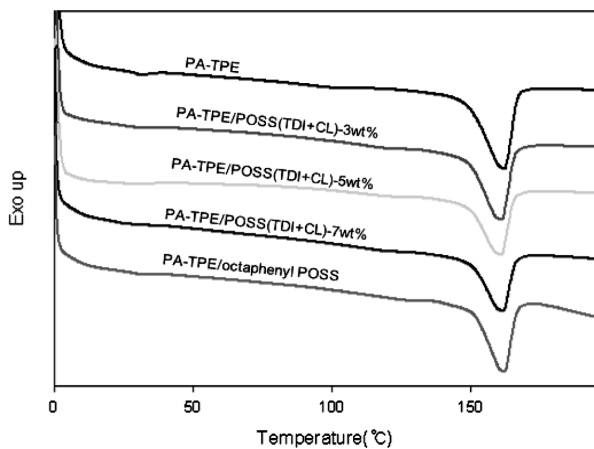
Figure 4. DSC thermograms of PA-TPE/POSS-(TDI+CL) composites with different POSS-(TDI+CL) contents and PA-TPE/octaphenyl POSS.
