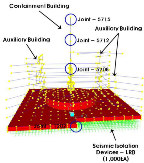
Fig. 5 3-D FE model(courtesy of KEPCO-E&C)
