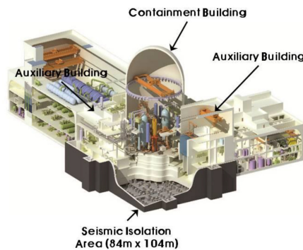
Fig. 4 Nuclear power plant with seismic isolation system(courtesy of KEPSCO-E&C)
