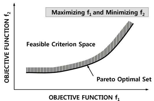
Fig. 2 Pareto solution set of multi-objective optimization with maximizing f_1 and minimizing f_2
