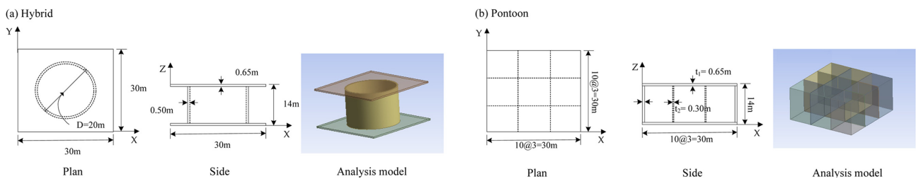
Fig. 2. Shape and dimension of unit module in each large floating structure.
