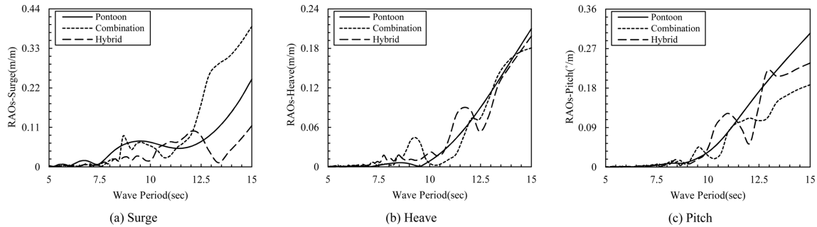
Fig. 10. Comparison of RAOs at each floating structure due to incidence wave angle 45^\circ .
