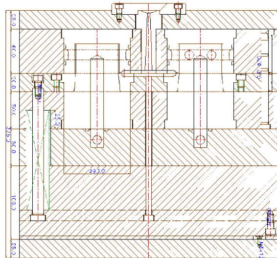
Figure 1. Mold design for 2-cavity injection molding.
