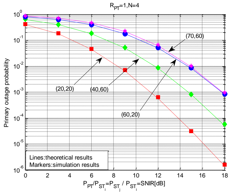
Fig. 6. Outage probability of the primary network with the varying position of the active secondary transmitter. Inactive secondary transmitters (relay sets) are located at (60, 40).
