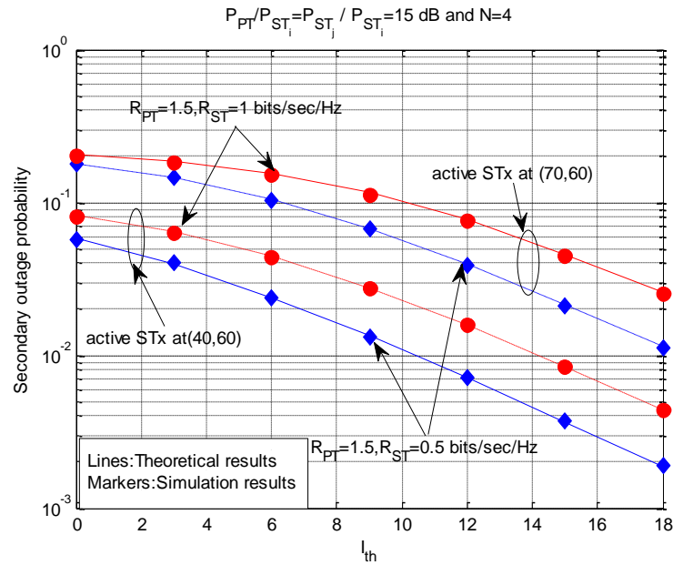
Fig. 8. Outage probability of the secondary network in SII.
