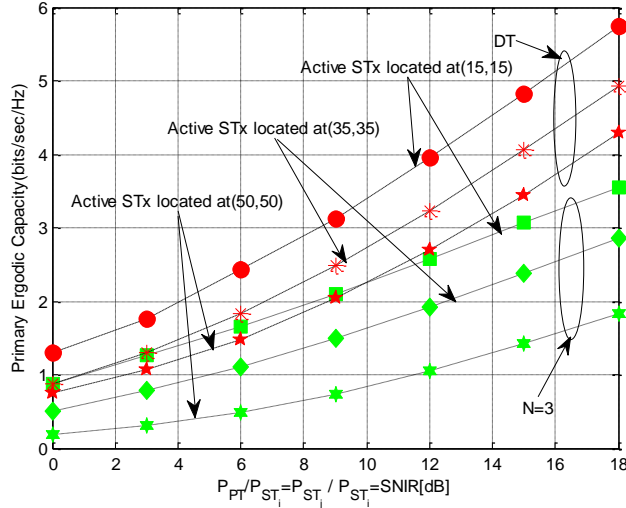
Fig. 4. Impact of the position of active secondary transmitter with respect to PRx. Inactive secondary transmitters (relay sets) are located at (60, 60).
