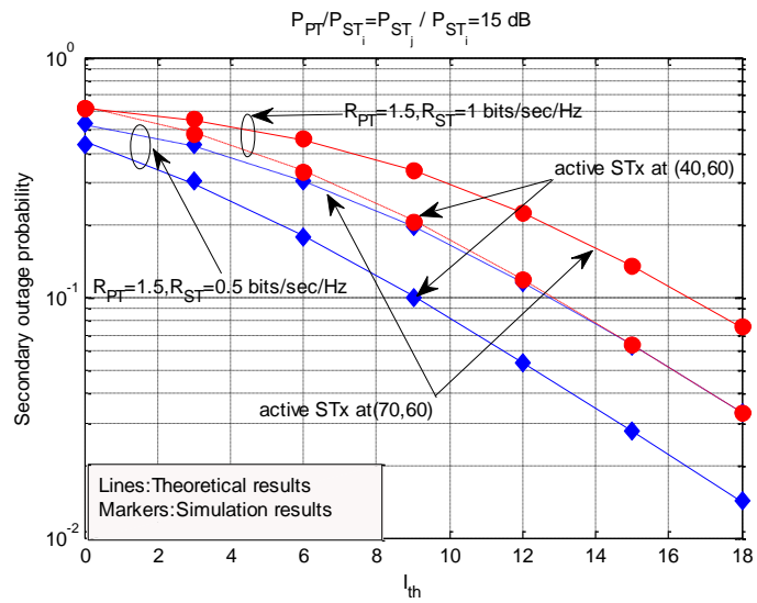
Fig. 7. Outage probability of the secondary network in SI.
