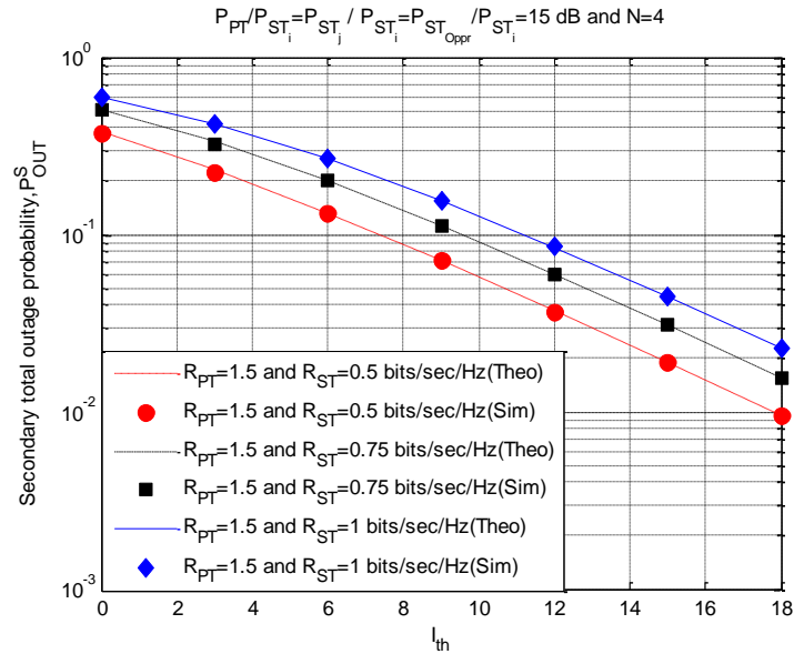
Fig. 10. Total outage probability of the secondary network.
