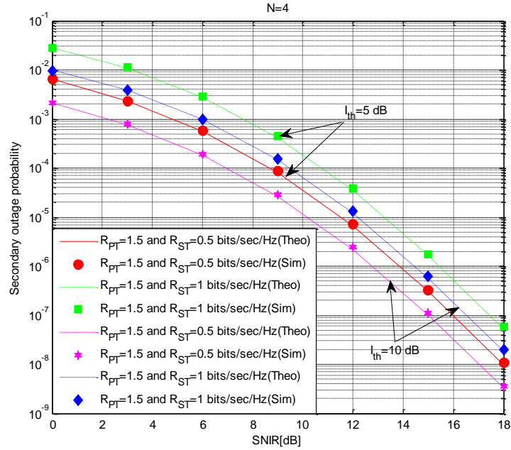
Fig. 9. Outage probability of the secondary network in SIII.
