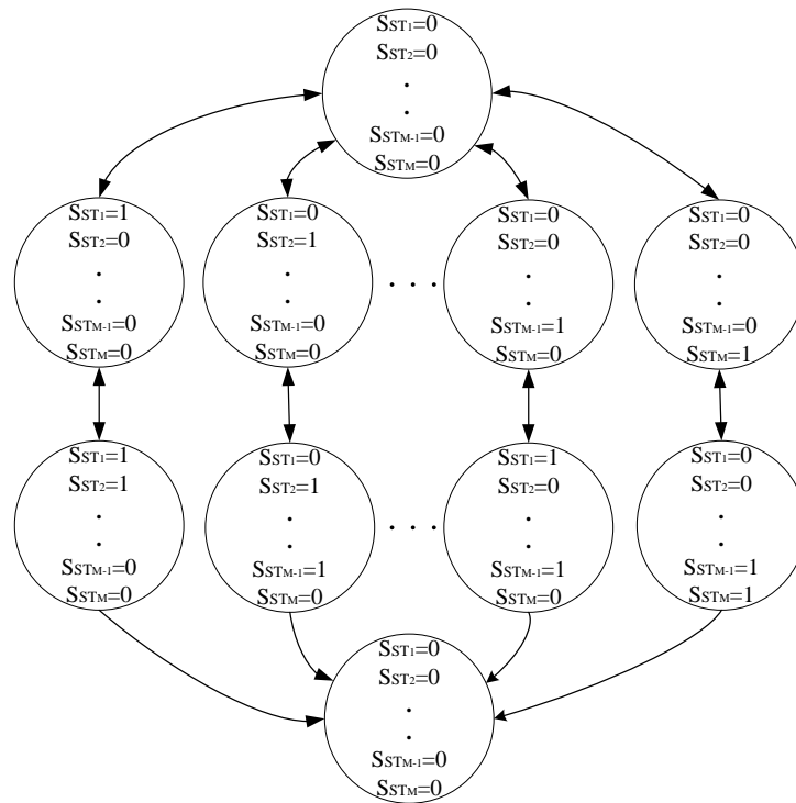
Fig. 2. General state transition scenario of the CR Transmitter (STx) of our proposed spectrum sharing model.
