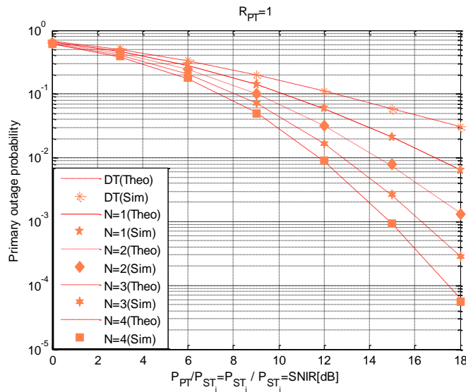
Fig. 5. Outage probability of the primary network. Active secondary transmitter is located at (30, 30) and inactive secondary transmitters (relay sets) are located at (50, 40).
