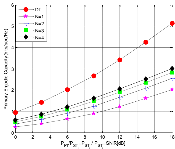
Fig. 3. Primary ergodic capacity with cooperative secondary user selection when the active secondary transmitter is located at (30, 30) and inactive secondary transmitters (relay sets) are located at (50, 50).
