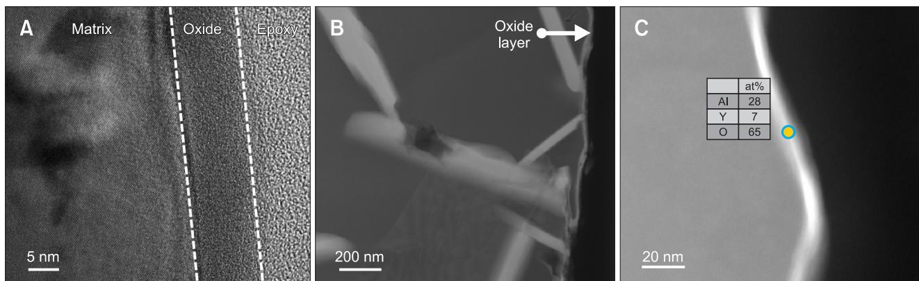
Fig. 1. Transmission electron microscope (TEM) images obtained from suction-cast \text{Al}_{87}\text{Ni}_3\text{Y}_{10} continuously heated up to 873 K. (A) High-resolution electron microscope image. (B) Lower magnification high-angle annular dark-field scanning TEM (HAADF-STEM) image. (C) Higher magnification HAADF-STEM image and energy dispersive spectrometer result.
