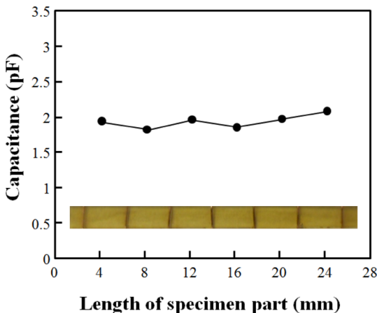
Fig. 5. Capacitance of epoxy resin for each section
