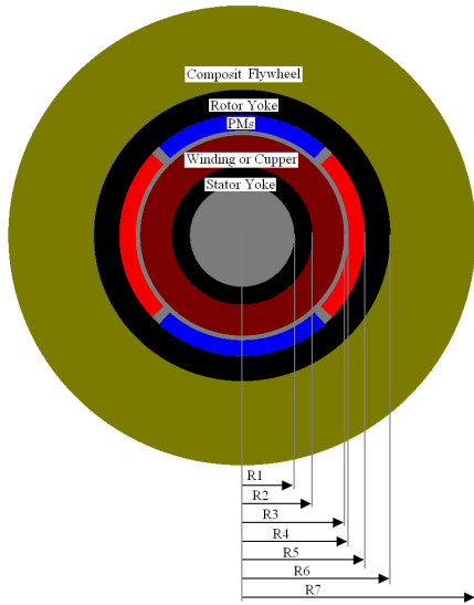
Fig. 1. Structure for micro-satellite EMB's: a hollow cylinder with centered external rotor electrical machine
