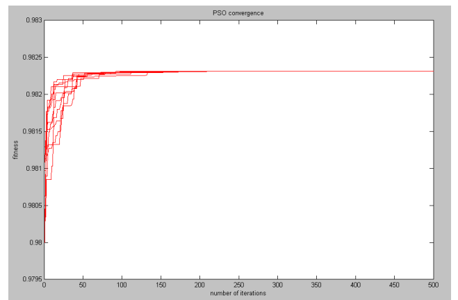
Fig. 4. Optimization results for ten run
