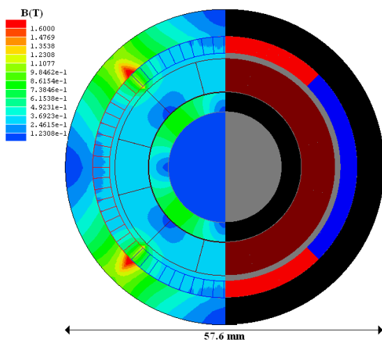
Fig. 5. Magnetic flux density distribution resulted by magneto-static simulation
