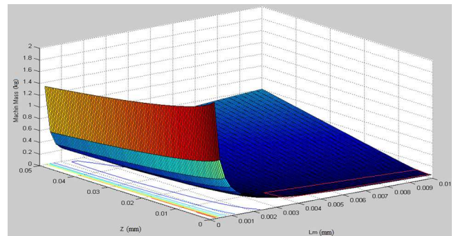
Fig. 3. Behavior of weight regard to variation of L_m and Z at constant B_p ( B_p=0.9T ).
