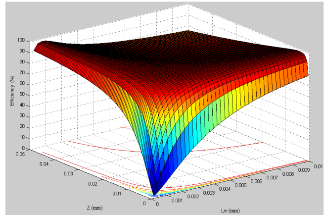
Fig. 2. Behavior of efficiency regard to variation of L_m and Z at constant B_{air} ( B_{air}=0.9T ).
