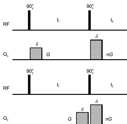
Figure 1. Two variations of the CRAZED pulse sequence depending on the position of the first encoding gradient pulse (top: at the beginning of the t_1 period; bottom: at the end the t_1 period).
