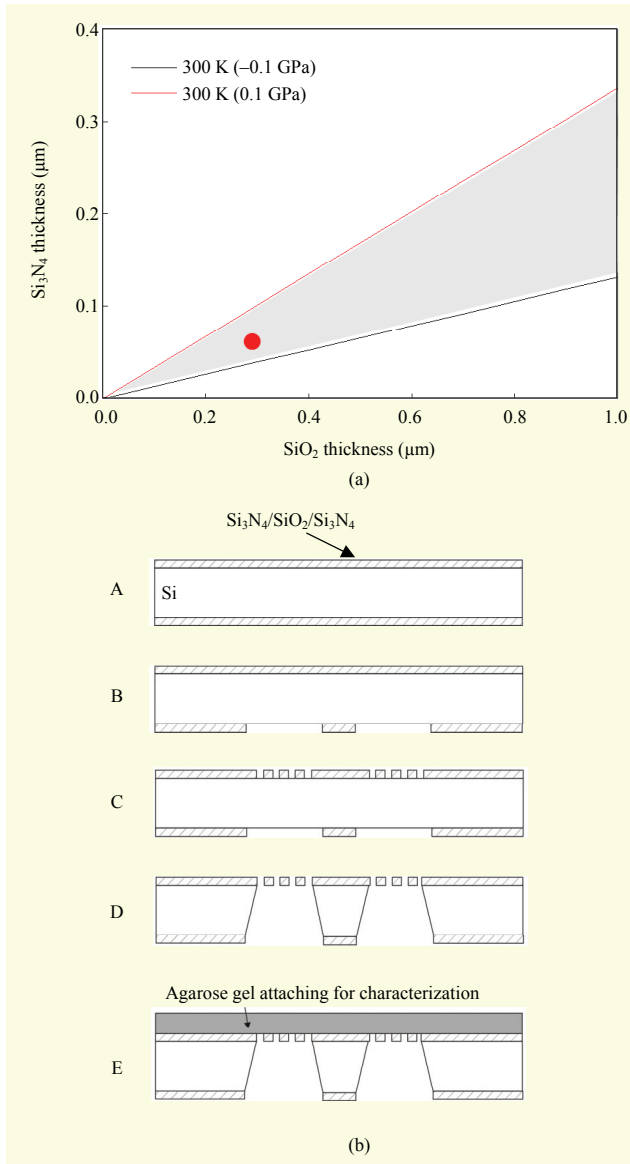
Fig. 2. (a) Calculation of Si 3 N 4 thickness (top plus bottom layers) vs. SiO 2 thickness to achieve |\sigma| < 0.1 GPa and (b) sequential procedures for fabrication of Si 3 N 4 /SiO 2 /Si 3 N 4 membrane sieves.
