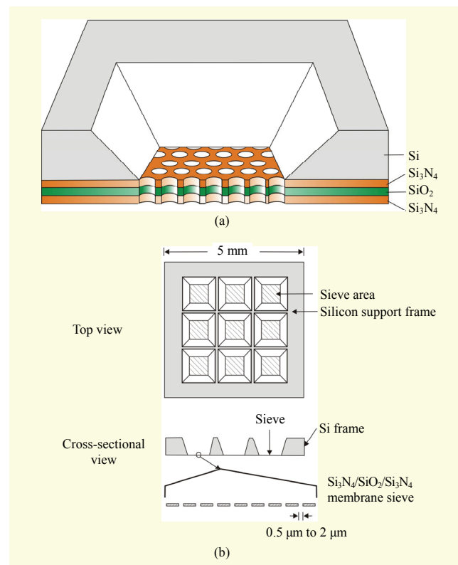
Fig. 1. Schematic diagram showing working principles of (a) \text{Si}_3\text{N}_4/\text{SiO}_2/\text{Si}_3\text{N}_4 membrane filter and (b) its structures.
