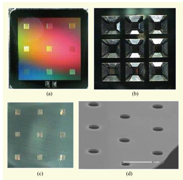
Fig. 3. Photographs of Si 3 N 4 /SiO 2 /Si 3 N 4 membrane filter (5 mm× 5 mm): (a) top membrane part, (b) bottom well part, (c) top membrane attached with agarose gel, and (d) magnified views on membrane sieves with 2-μm diameter.
