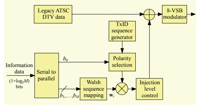
Fig. 5. Block diagram of proposed scheme.
