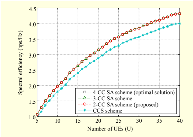
Fig. 2. Spectral efficiency vs. number of UEs (U).
